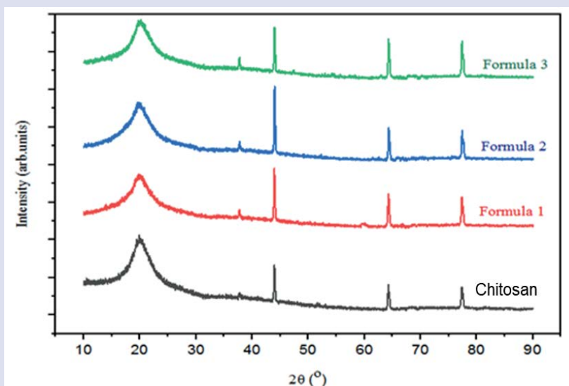
Figure 3: X-Ray Diffraction Spectra of Chitosan (—), Formulatin I (—), Formulation 2 (—), Formulation 3 (—).
