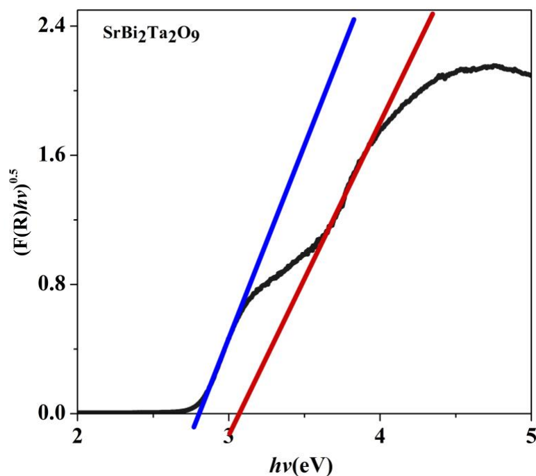
Figure 5. Tauc-plot of band gap energy of \text{SrBi}_2\text{Ta}_2\text{O}_9 compound
