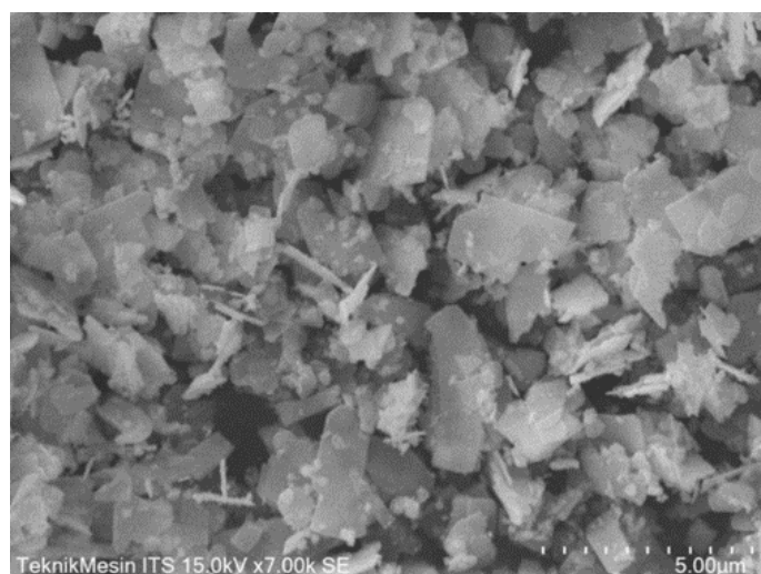
Figure 2. Micrograph of \text{SrBi}_2\text{Ta}_2\text{O}_9 compound
