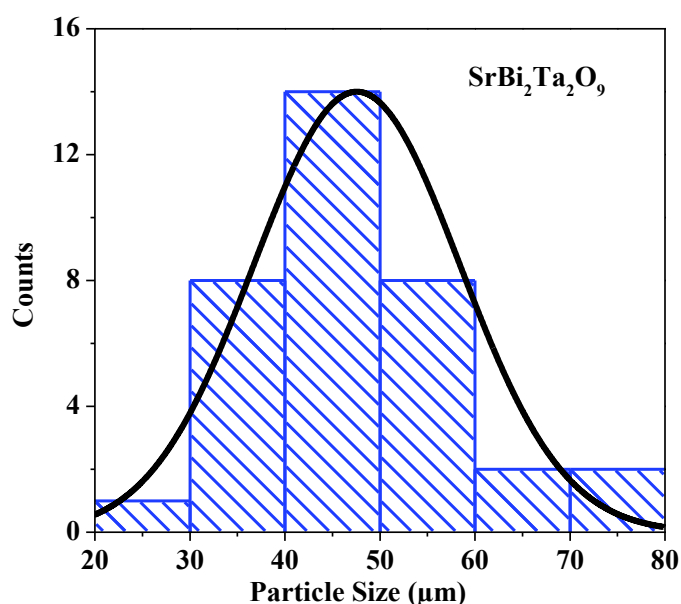
Figure 3. Particle size distribution of \text{SrBi}_2\text{Ta}_2\text{O}_9 compound
