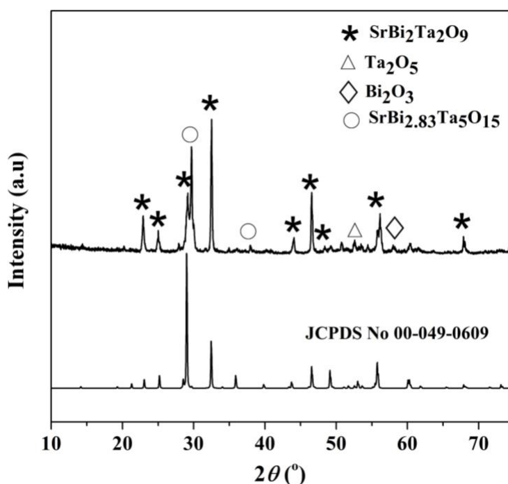
Figure 1. \text{SrBi}_2\text{Ta}_2\text{O}_9 diffractogram
