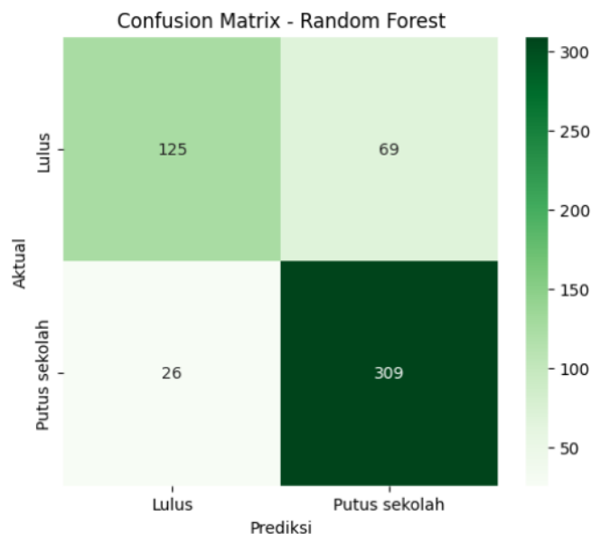
Figure 6. Confusion Matrix for Scenario 3
