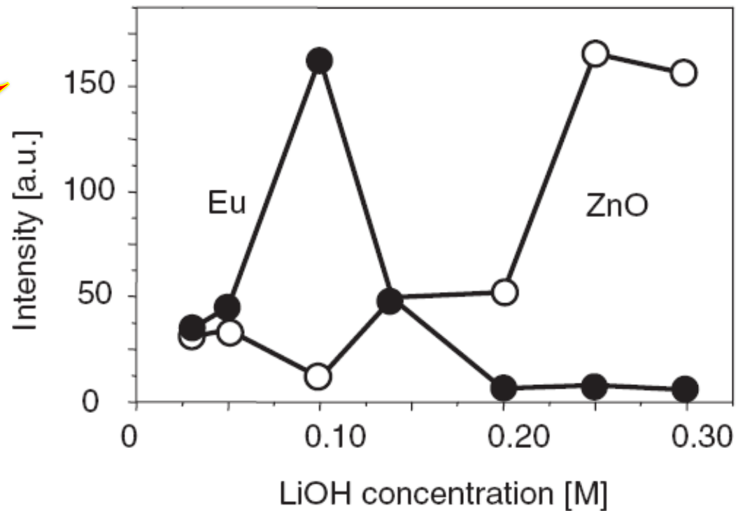
Fig. 6. Effect of [LiOH] on the visible luminescence intensity of ZnO (open circles) and red luminescence intensity (closed circles) of ZnO-Eu/PEG samples prepared at Eu/Zn = 0.08:1 mol/mol.
