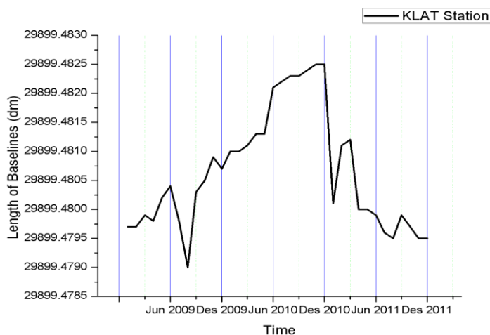
Figure 8. The change of baseline in KLAT station
