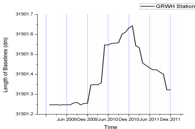
Figure 7. The change of baseline in GRWH station
